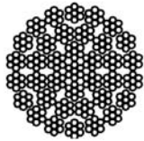
500 MCM CLASS "G" 259 STRANDS
